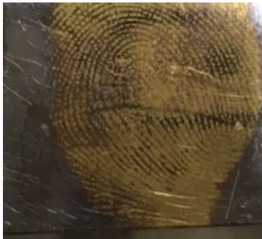
FIG. 3—Fingerprint developed with vacuum metal deposition (gold/zinc) on brass surface.
