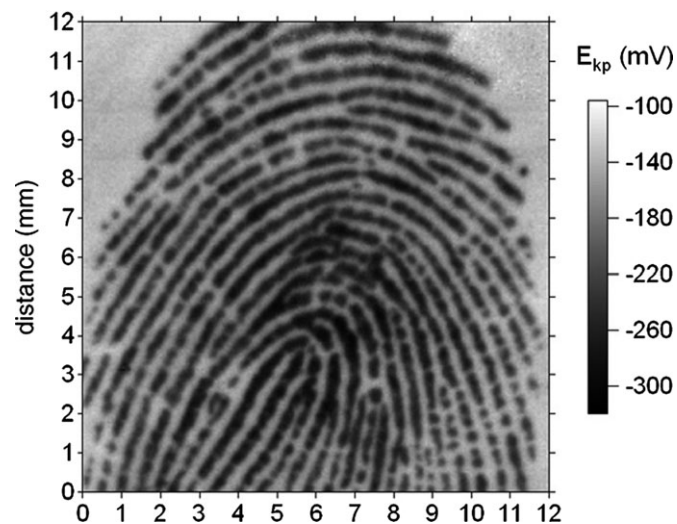
FIG. 1—Image created by scanning Kelvin Probe on iron substrate (27).
